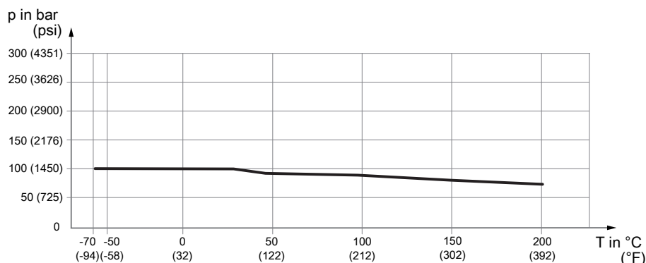
Fig. 17: Allowed process pressure as a function of temperature, suitable for process connection temperature, suitable for process connections with internal thread G and NPT
