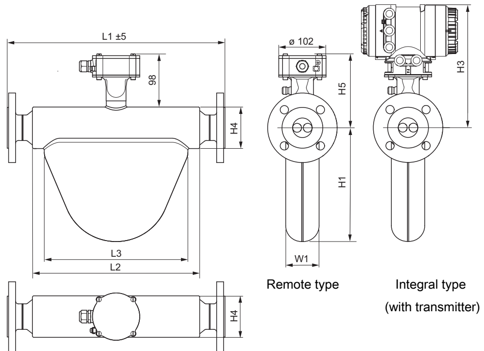
Fig. 21: Dimensions in mm
