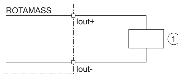
Fig. 24: Active current output connection lout HART
