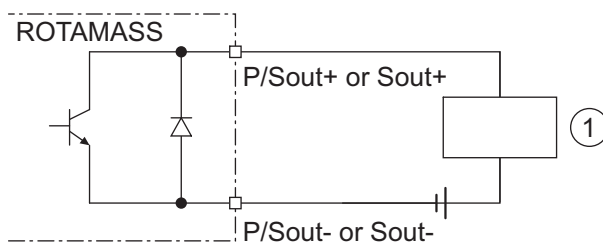
Fig. 34: Passive status output connection P/Sout
