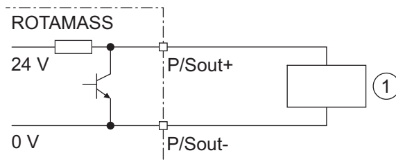
Fig. 29: Active pulse output P/Sout with internal pull-up resistor
