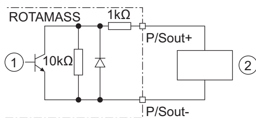
Fig. 36: Passive pulse or status output with switching amplifier connected in series
