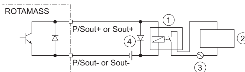
Fig. 35: Passive status output connection P/Sout for solenoid valve circuit
