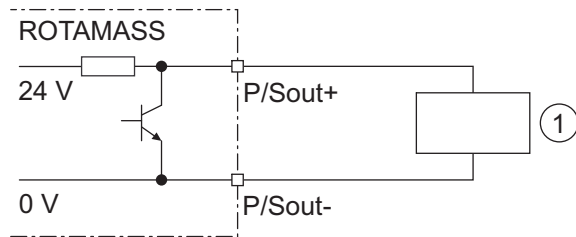
Fig. 33: Active status output P/Sout with internal pull-up resistor
