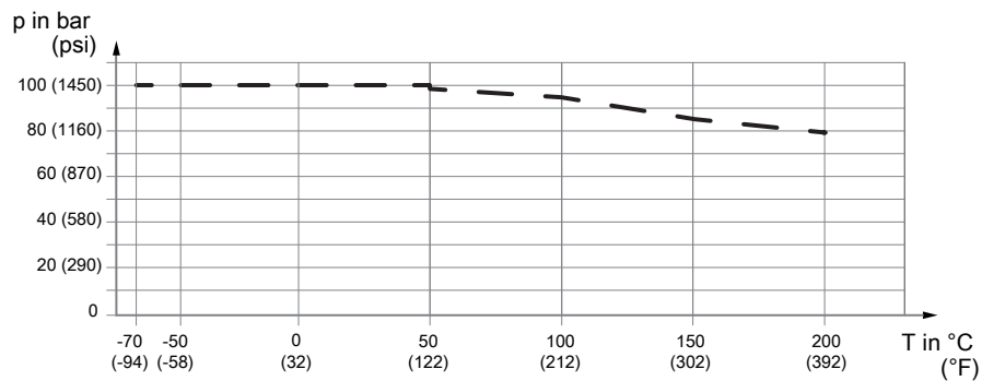
Fig. 15: Allowed process pressure as a function of process connection temperature, suitable for flange EN 1092-1 PN100
