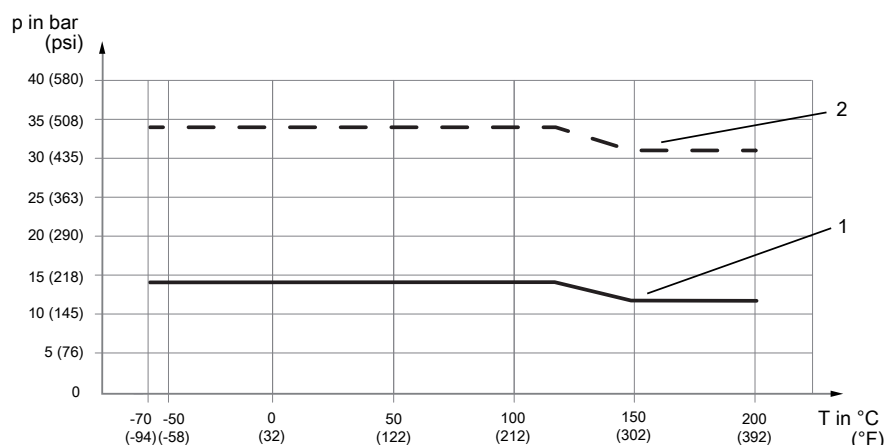
Fig. 16: Allowed process pressure as a function of process connection temperature
