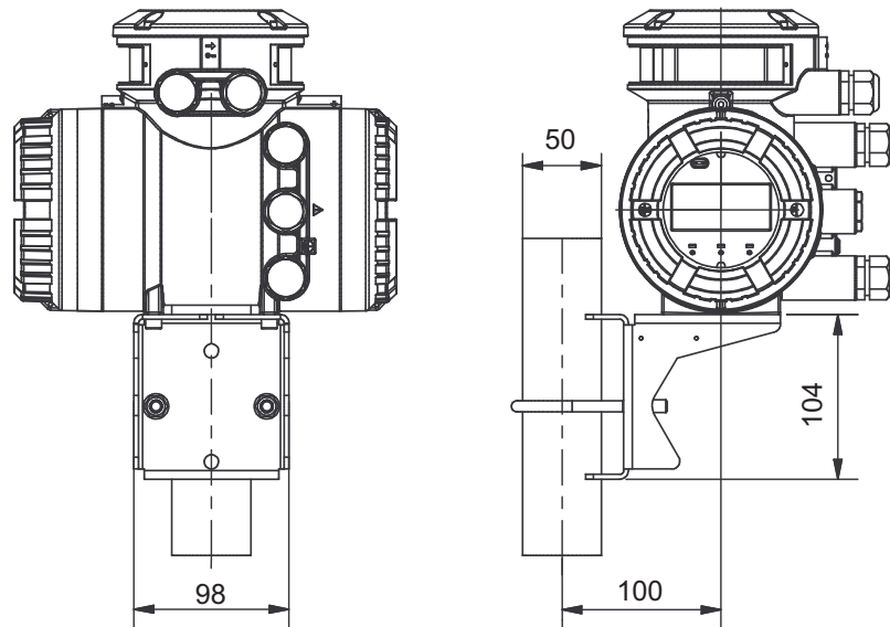
Fig. 23: Dimensions of transmitter in mm, attached by sheet metal console (bracket)
