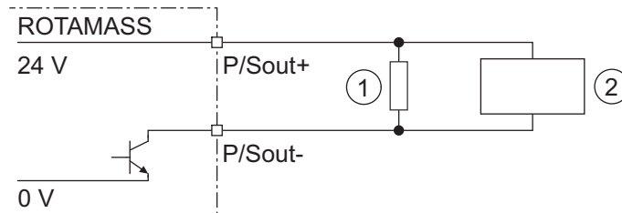
Fig. 27: Active pulse output connection P/Sout
