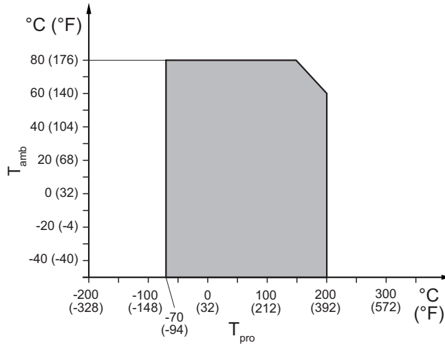
Fig. 19: Allowed medium and ambient temperatures, remote type
