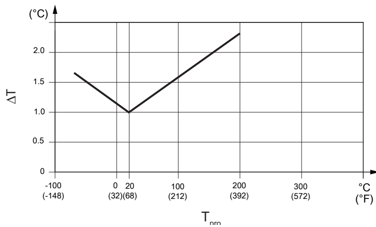
Fig. 10: Temperature accuracy
