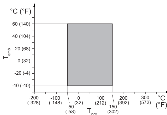
Fig. 18: Allowed medium and ambient temperatures, integral type
