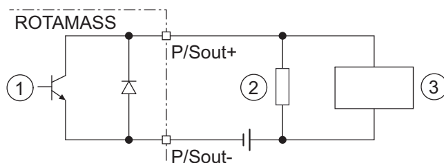
Fig. 30: Passive pulse output connection P/Sout with electronic counter
