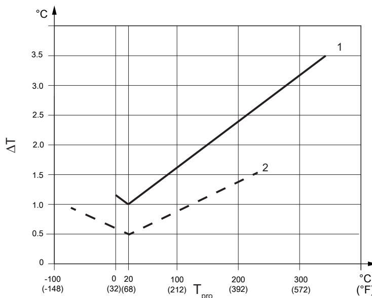
Fig. 11: Temperature accuracy
