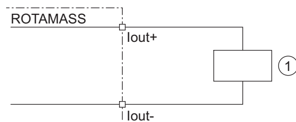
Fig. 28: Active current output connection lout HART
