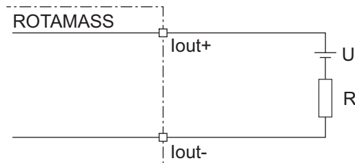
Fig. 30: Passive current output connection I out
