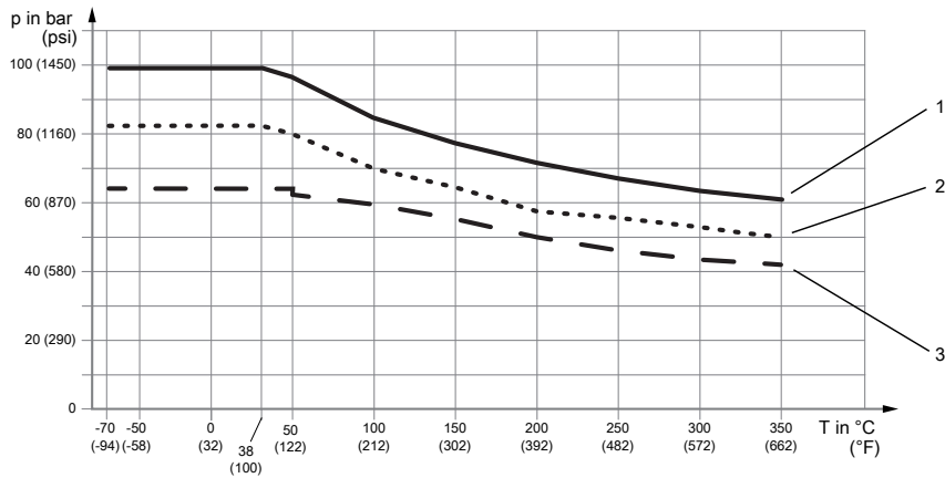
Fig. 15: Allowed process pressure as a function of process connection temperature
