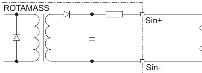
Fig. 43: Status input connection
