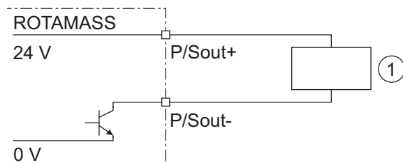
Fig. 36: Active status output connection P/Sout
