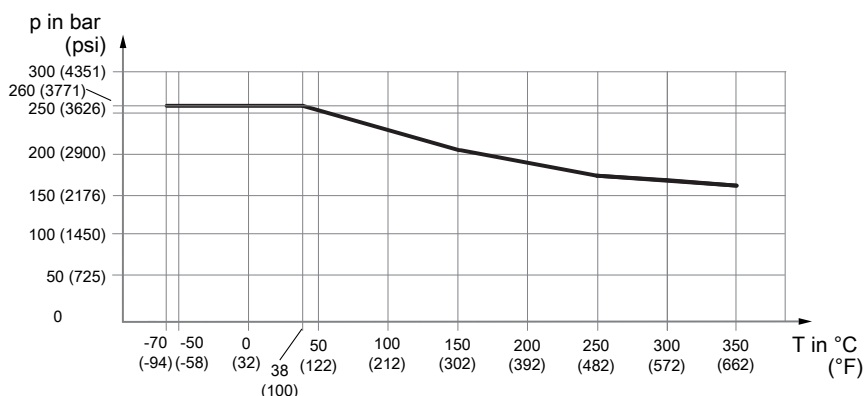
Fig. 18: Allowed process pressure as a function of temperature, suitable for process connection temperature, suitable for process connections with internal thread G and NPT
