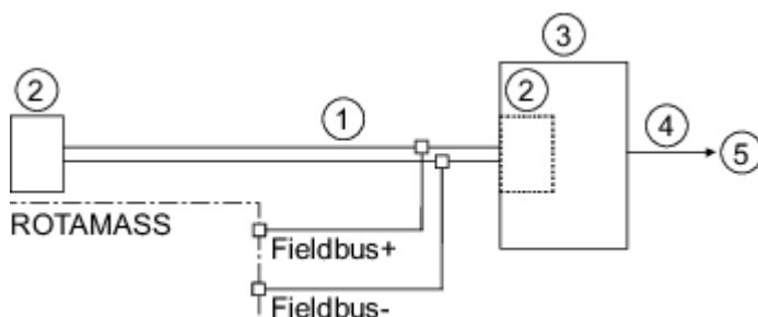
Fig. 35: Raccordement PROFIBUS PA
